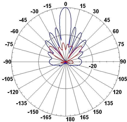
Azimuth Radiation Pattern Midband Freq. 5.25 GHz
