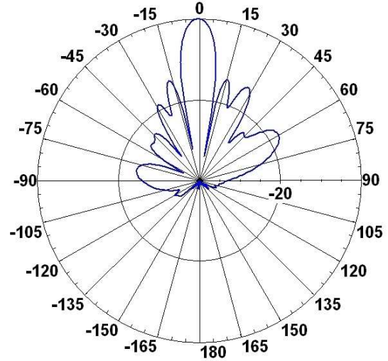
Elevation Radiation Pattern Midband Freq. 5.25 GHz
