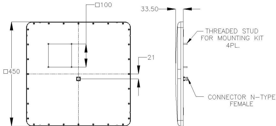
Dimensions [mm]
