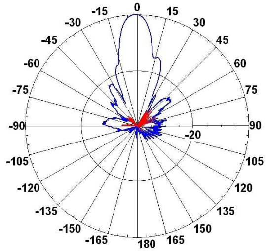
Elevation Radiation Pattern Midband Freq. 3.3 GHz
