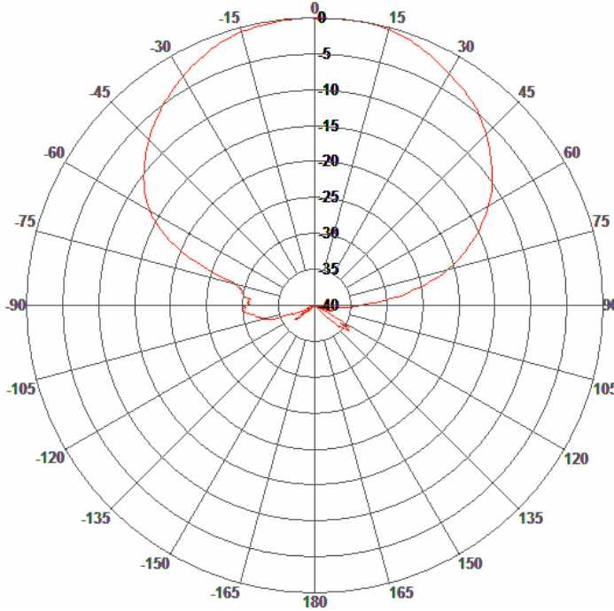
E-Plane Pattern
