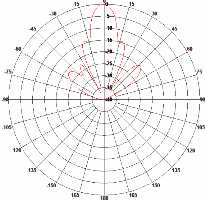
E-Plane Pattern
